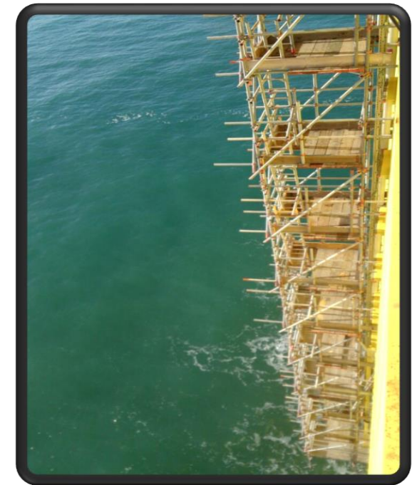
24m Hanging Scaffold
