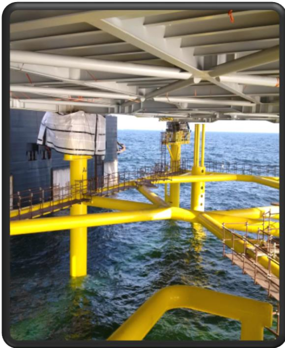
Spiderdeck Walkways
