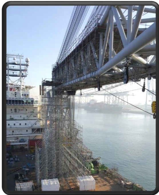
Maintenance Heavy Lift Crane
