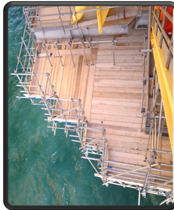
Heavy Load Scaffold 500kg/m 2
